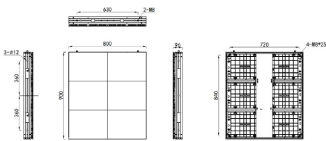
Figure 1 Drawing of Front Maintenance Cabinet
