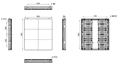
Figure 2 Drawing of Rear Maintenance Cabinet
